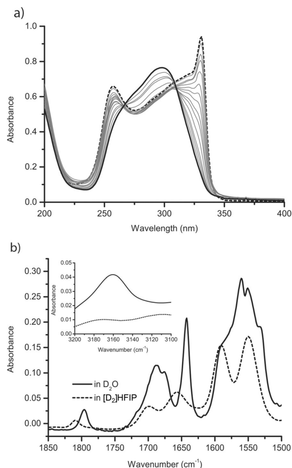
Figure 3. a) UV/Vis spectrum of 1 in water (0.005 wt%) as a function of HFIP concentration. b) IR spectrum recorded in the amide I region and amide II in \text{D}_2\text{O} and [\text{D}_2]\text{HFIP} . Inset: N–H and C–H stretch region.
